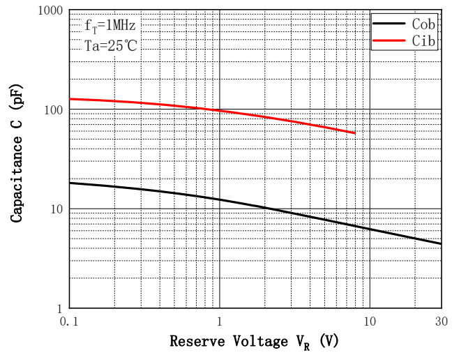
Fig. 6 - C_{ob}/C_{ib} - V_{CB}/V_{EB}
